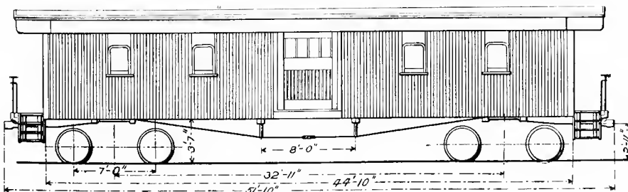
Fig. 87. Side Elevation.
